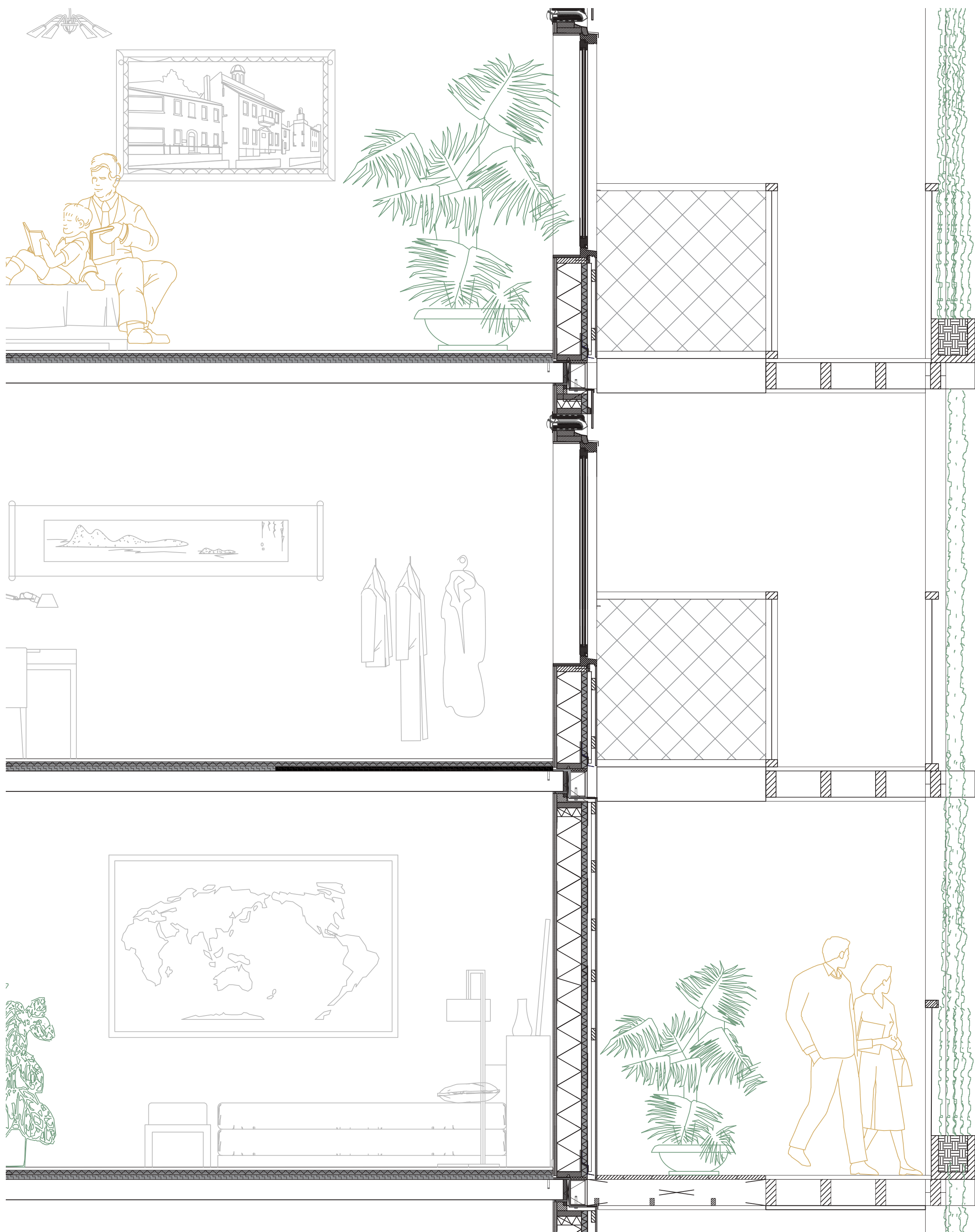
Vertical section 1:20
