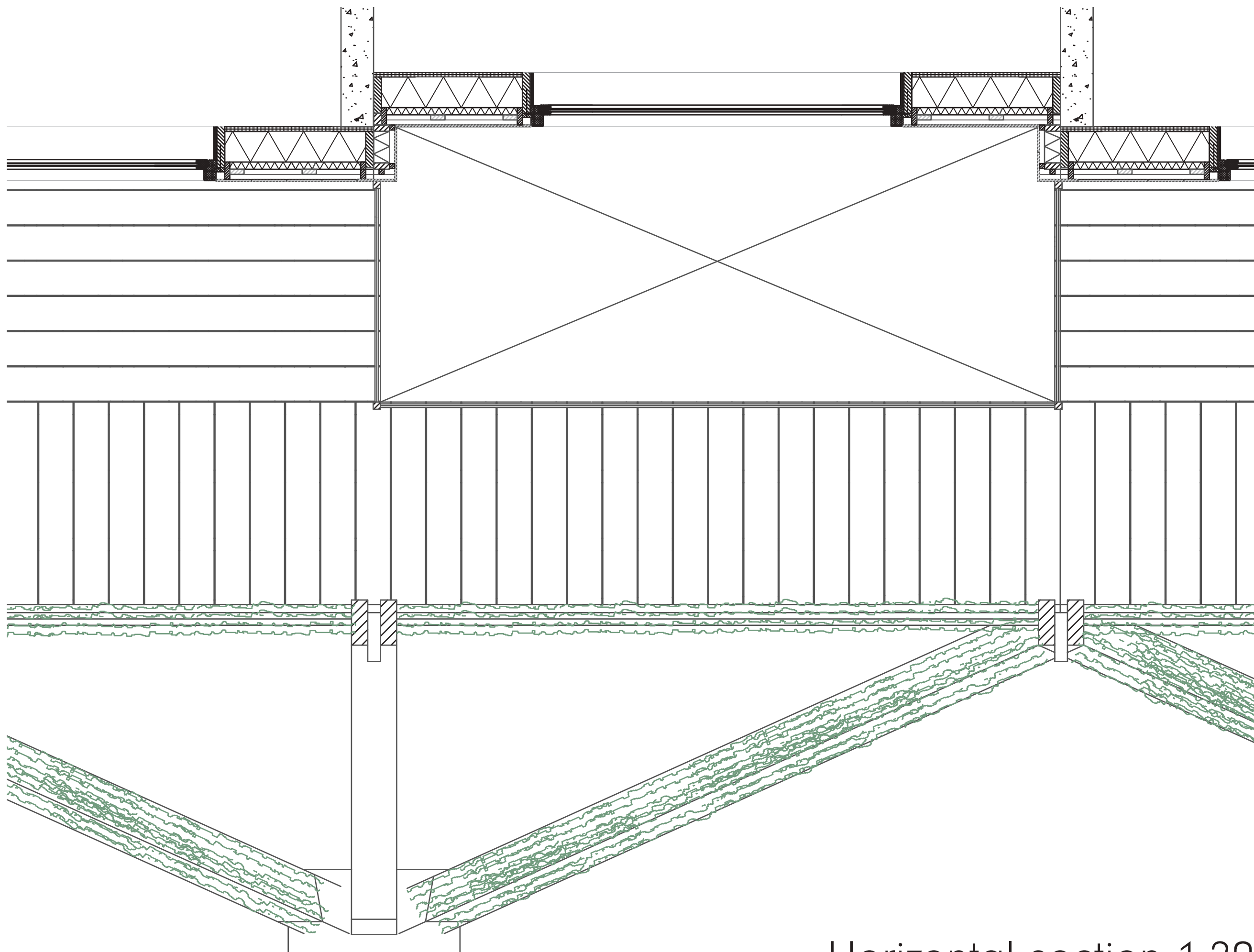
Horizontal section 1:20
